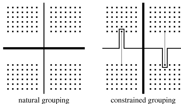
Fig. 3. Undesired grouping from sparse constraints. Left: In the 2-class grouping based on proximity, the horizontal division is optimal while the vertical division is suboptimal. Right: When we add constraints that the points linked together have to belong to the same group, the vertical division becomes the desired partitioning. However, the slightly modified horizontal division is a partitioning that satisfies the constraints, while producing the maximum objective value \varepsilon .
