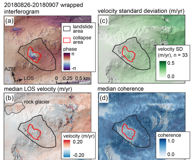
Figure 4. InSAR-derived LOS velocity of the landslide prior to the 28 June collapse. Interferograms come from Sentinel-1 ascending track 151. (a) A wrapped interferogram from the summer of 2018 showing clear landslide deformation of roughly 10 cm in 12 d. (b) Median LOS velocity of the failure area and landslide area. Interferograms with short temporal baselines and high median coherence on the landslide slope were used to create the velocity map. Positive values (red) correspond to motion away from the satellite along the satellite LOS. Note the spatial inconsistency of signals within the landslide. Negative velocity values at lower elevations are caused by topography-correlated atmospheric noise. (c) Standard deviation of LOS velocity. (d) Median coherence of the failure area and landslide area.
