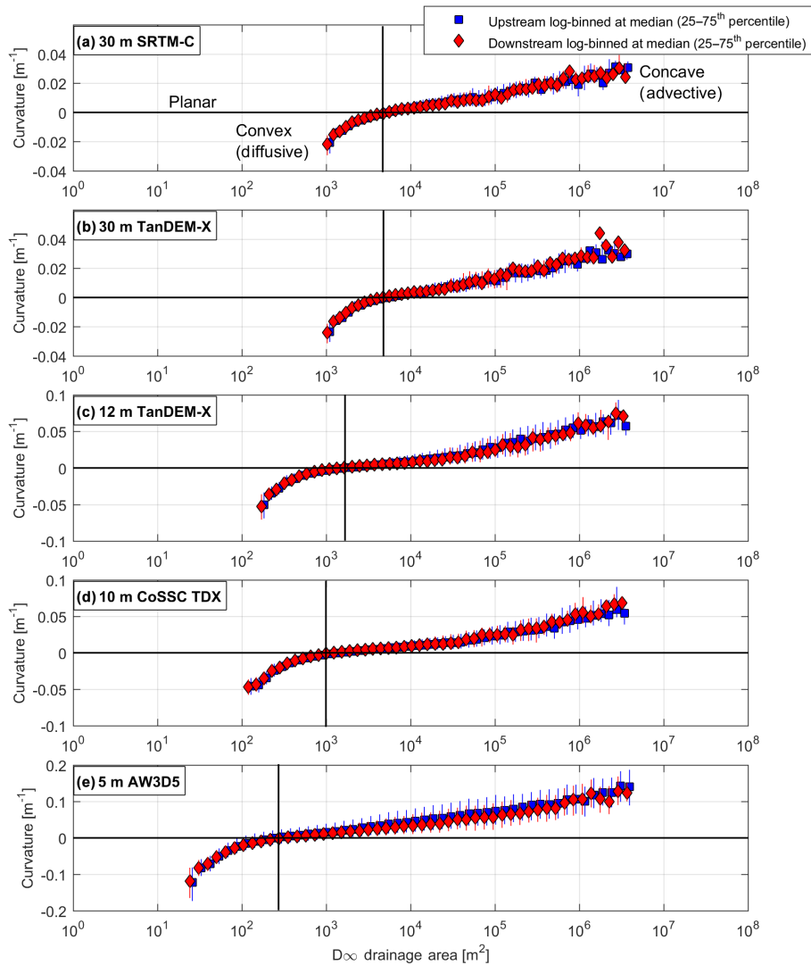
Figure 10. Logarithmically binned drainage area versus median curvature with 25–75th percentile range of curvatures indicated for (a) SRTM-C 30 m, (b) TanDEM-X 30 m, (c) TanDEM-X 12 m, (d) CoSSC TDX 10 m, and (e) AW3D5 5 m DEMs. Analysis separated downstream (red diamonds) and upstream (blue squares) of the knickpoint. Greater variability in curvature (larger error bars and greater y-axis range) is measured in the 5 m data. Vertical line marks approximate changeover from diffusive hillslope processes (convex curvature) to advective fluvial processes (concave curvature).
