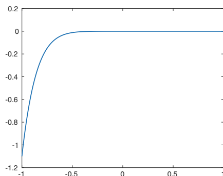
FIG. 1. Plot of the denominator of the rational interpolant whose roots were computed to produce the eigenvalue approximations in Table 1.
