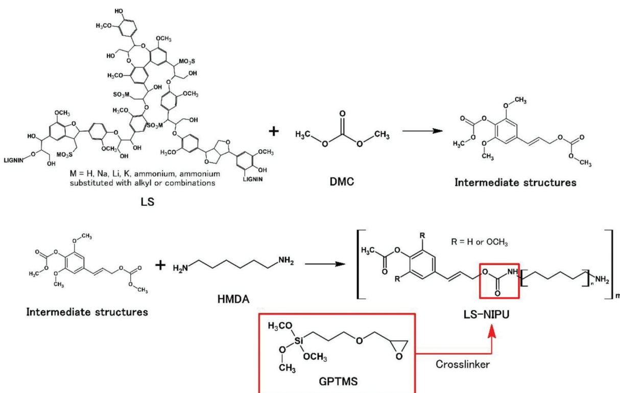
Figure 8: Synthesis mechanism of LS-NIPU
