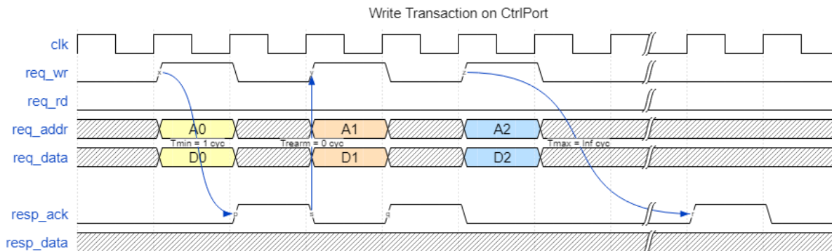
Figure 4: ctrlport write transaction
