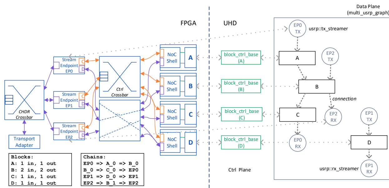
Figure 17: Example FPGA and SW objects in an RFNoC graph
