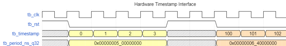
Figure 15: An example of a time-base reconfiguration from 200 MHz to 160 MHz
