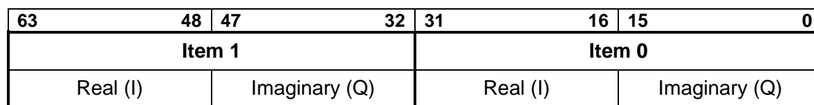
Figure 9: 64-bit bus with SC16 data items
