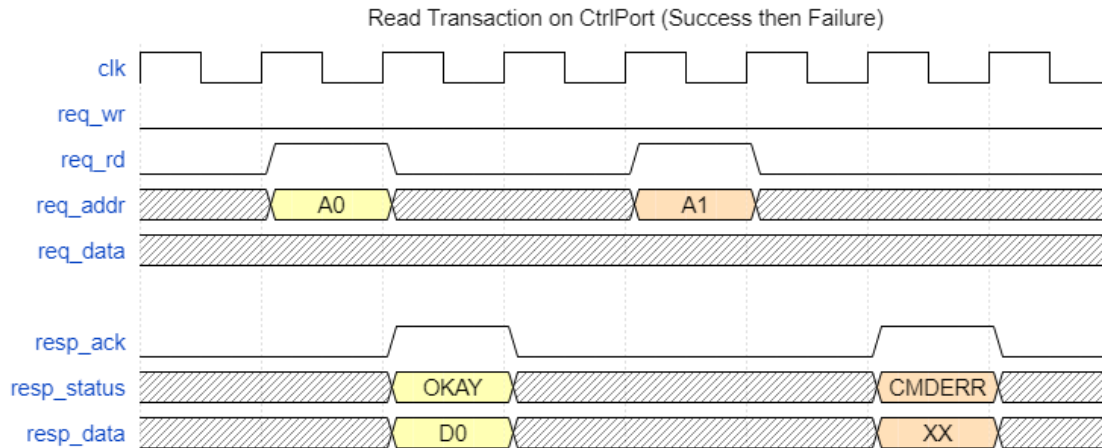
Figure 6: Read completion status (Success and Failure)
