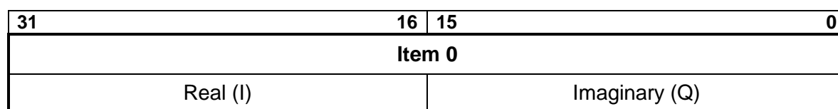
Figure 8: 32-bit bus with SC16 data items
