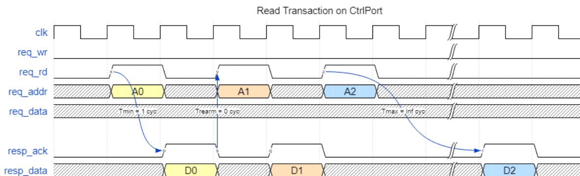
Figure 5: ctrlport read transaction
