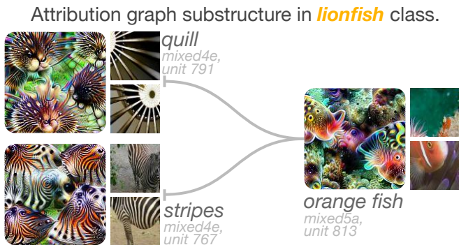
Fig. 7. An example substructure from the lionfish attribution graph that shows unexpected texture features, like “quills” and “stripes,” influencing top activated channels for a final layer’s “orange fish” feature (some lionfish are reddish-orange, and have white fin rays).
