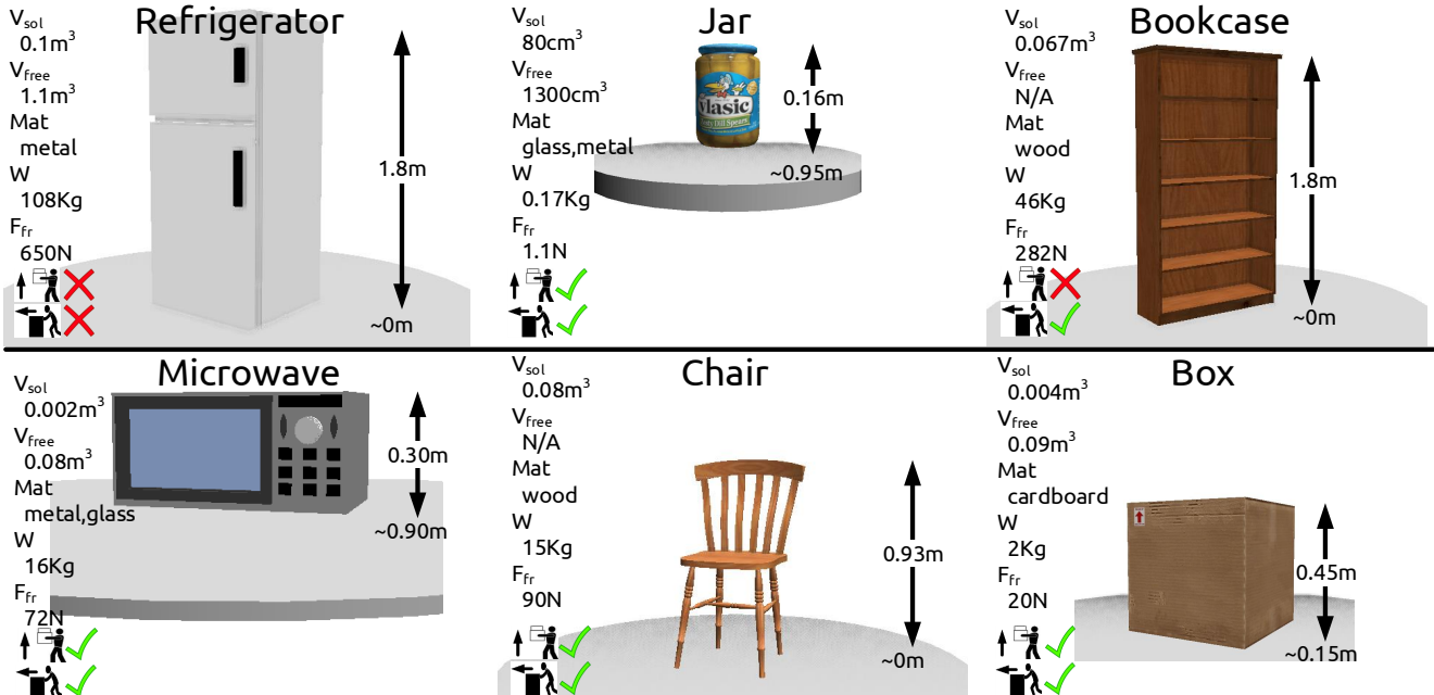
Figure 2. By jointly using estimates of the dimensions, static support surface height, material composition, and solidity of objects we estimate occupied and free container volume ( V_{sol} and V_{free} ), weight W , and static support friction F_{fr} forces of objects. This allows us to make predictions such as whether it would be easy for people to carry or push each object instance (indicated by symbols at bottom).
