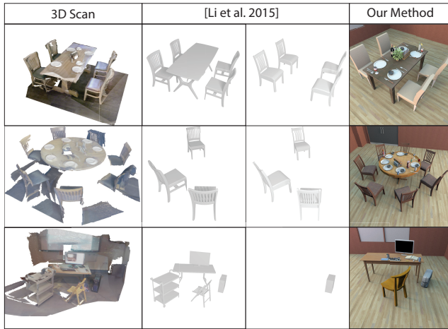
Figure 12: Retrieval results using [Li et al. 2015]. In the second column, we show the results using a 6,000 model database specifically tailored to contain the models in the scan. In the third column, we show the results using our 12,000 model database containing more general indoor objects. Geometric retrieval methods often fail when insufficient key points can be extracted (e.g., the round table and the small items on the table) or the extracted key points cannot form consistent constellations due to partial scan or occlusions (e.g., the chairs with only the upper parts scanned).
