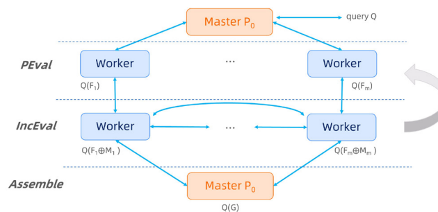
Figure 8: Execution model in GAE
