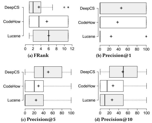
Figure 8: The statistical comparison of FRank and Precision@k for three code search approaches
