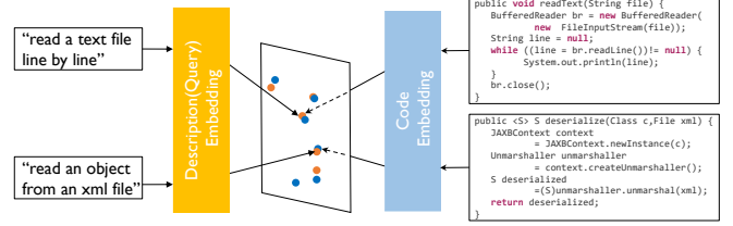
Figure 3: An example showing the idea of joint embedding for code and queries. The yellow points represent query vectors while the blue points represent code vectors.
