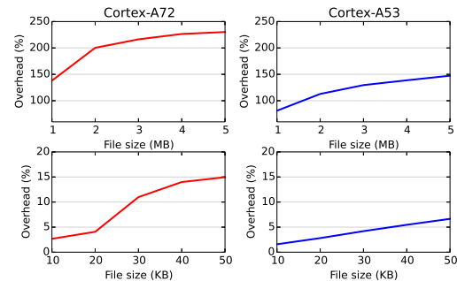
Figure 9: The performance overheads of SMOKEBOMB-protected 7zip application.
