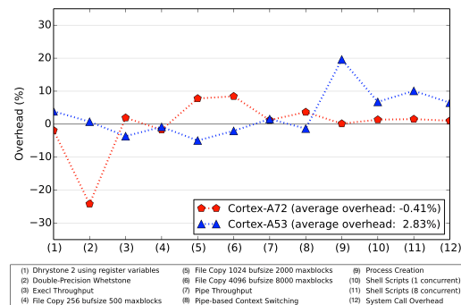
Figure 10: The performance overheads on each benchmark applications when SMOKEBOMB is activated.
