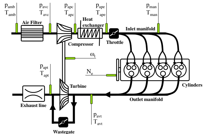
Figure 1. Air path sketch of a turbocharged SI engine ( p stands for pressure, T for temperature, N_e and \omega_t are respectively the engine and turbocharger rotational speed).
