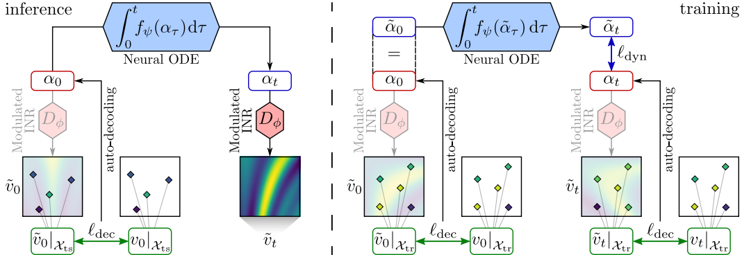
Figure 2: Proposed DINO model. Inference (left): given a new initial condition observed on a grid \mathcal{X}_{\text{ts}} , v_0|_{\mathcal{X}_{\text{ts}}} , forecasting amounts at decoding \alpha_t to \tilde{v}_t , by unrolling \alpha_0 with a time-continuous ODE dynamics model f_\psi . Train (right): given an observation grid \mathcal{X}_{\text{tr}} and a space-continuous decoder D_\phi , \alpha_t is learned by auto-decoding s.t. D_\phi(\alpha_t)|_{\mathcal{X}_{\text{tr}}} = v_t|_{\mathcal{X}_{\text{tr}}} ; its evolution is then modeled with f_\psi .
