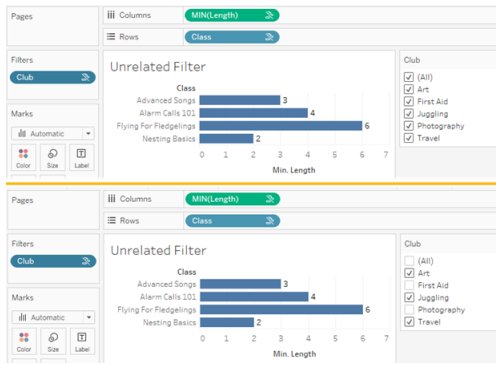
Two screenshots of viz with an unrelated filter, showing that deselecting options in the interactive filter control doesn't impact the viz
