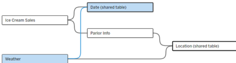
A multiple base table data model, with two unrelated tables (Ice Cream Sales and Weather) and two shared tables (Date and Location). There is an intermediate table, Parlor Info, between Ice Cream Sales and Location.
