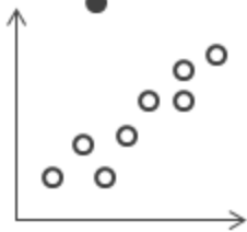
Outliers
