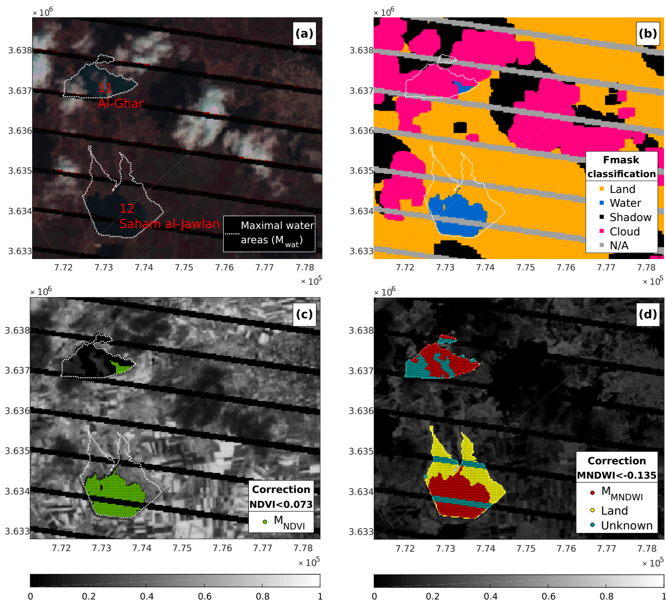
Figure 4. 2D dynamic water classification over a part of a Landsat 7 image (174/37) obtained on March 30 th , 2010. (a) SWIR-R-G image. Two reservoirs can be seen by eye – even if their appearance is very similar to cloud shadow areas –, but the hedges are not easy to detect due to the cloud cover. (b) Results of the Fmask classification. Water areas detection is not precise enough to directly use the results for the estimation of reservoirs surface area. (c) NDVI image. Water pixels’ low NDVI here contrasts with the surrounding irrigated crops’ high NDVI, as the two reservoirs are located close to cultivation areas. (d) MNDWI image. Red dots indicate water areas obtained after the 2D enhancement (Sect. 2.1). The 3D reconstruction is operated later (Sect. 2.3) on the Unknown part.
