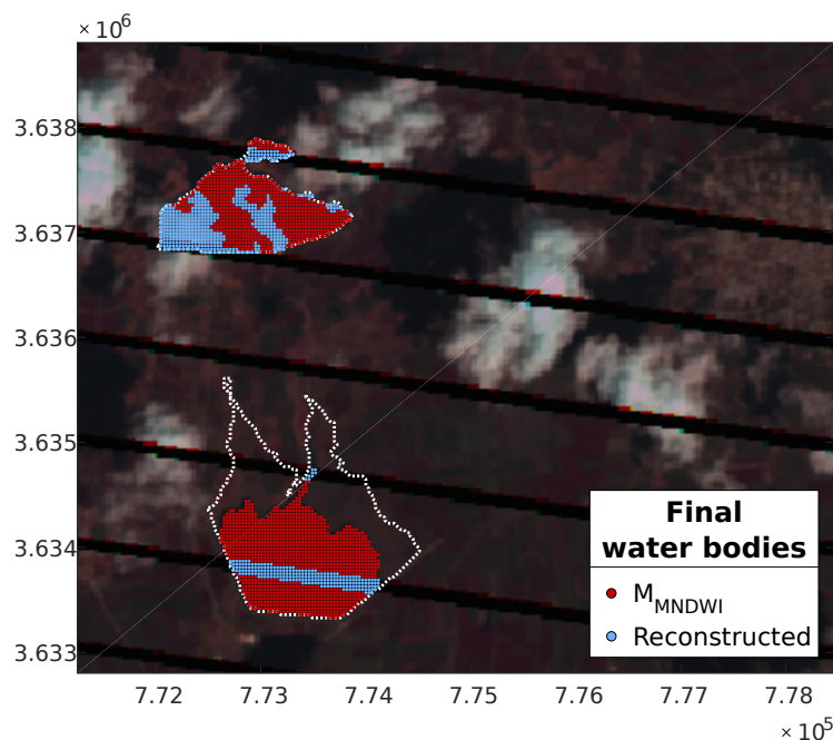
Figure 8. SWIR-R-G image. Final water bodies as obtained after the 2D enhancement and the 3D reconstruction applied to the Landsat 7 image (174/37) taken on March 30 th , 2010 (same as Fig. 4).
