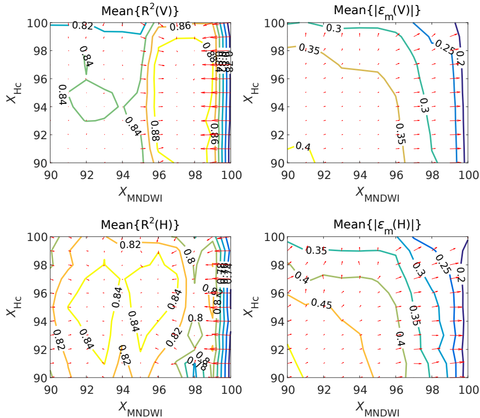
Figure 11. Sensitivity analysis of the two thresholds used to improve water bodies surface area estimates. Indices are averaged for all Jordanian reservoirs (except King Talal). Arrows point towards larger R^2 , or lower |\varepsilon_m| , and lengths are proportional to the gradient.
