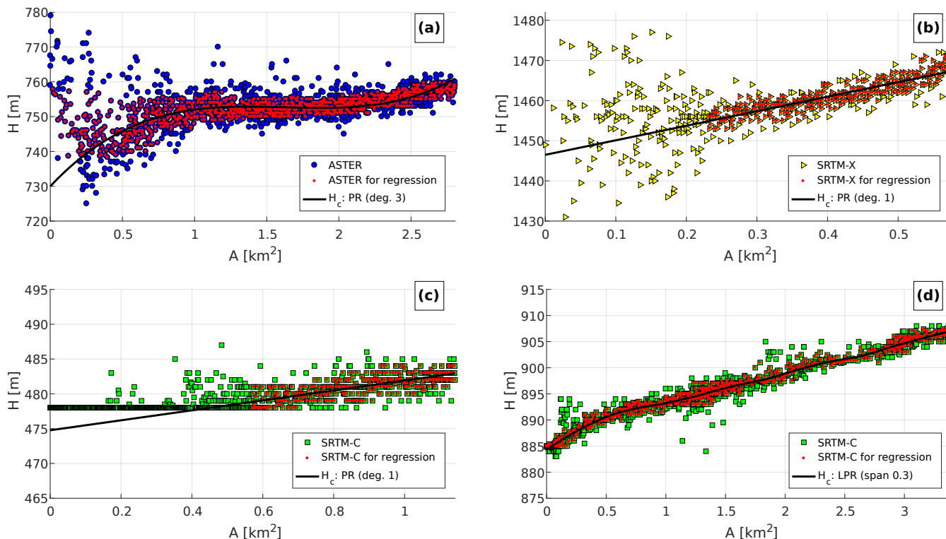
Figure 7. Elevation-area relationship and regression for a few reservoirs in the Yarmouk River Basin: (a) Kudnah, (b) Roum, (c) Al Ghar and (d) Qunaitera. Each symbol (circle, square or triangle depending on the DEM) represents the information associated to one pixel in a reservoir. PR and LPR stand for Polynomial Regression and Local Polynomial Regression respectively.
