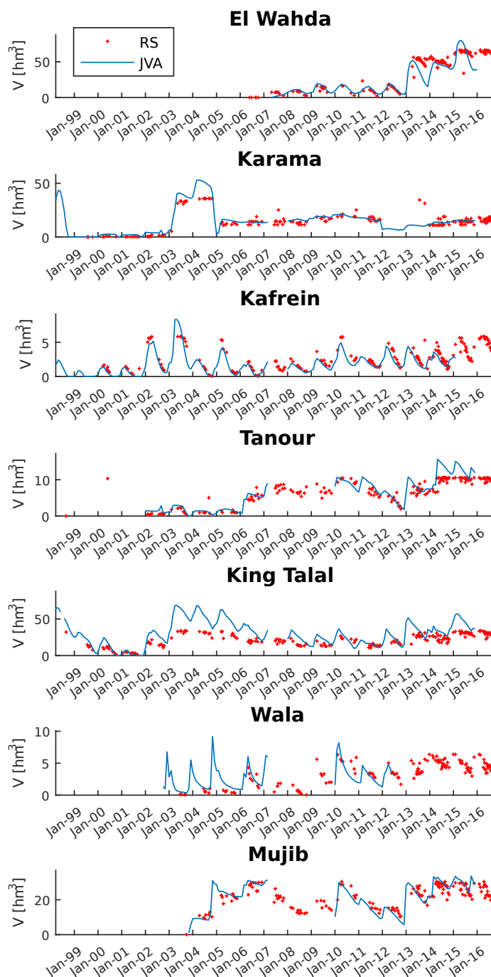
Figure 10. Storage variations for Jordan managed reservoirs. Red crosses indicate estimates from the method developed in this paper. The blue lines indicate in situ data records that were made by the Jordan Valley Authority (JVA).
