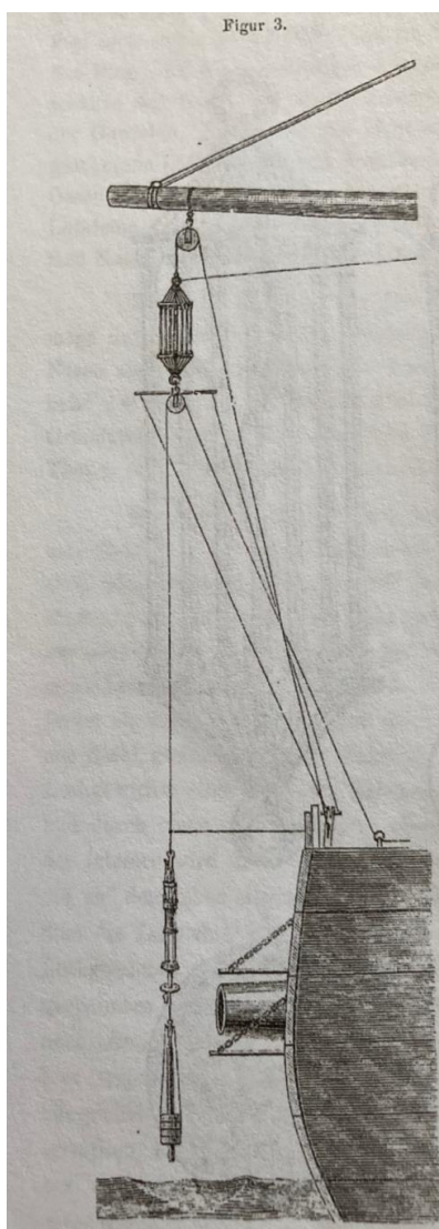
Figure 6: Reproduction of Figure 3 (page 16) of the Gazelle narrative showing the deployment of a Baillie sounder.
