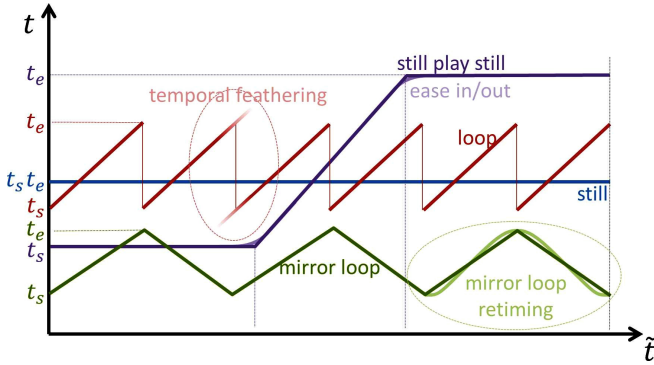
Figure 2: Various cliplet layer types graphed using input video time t as a function of output cliplet time \tilde{t} . Subscripts s and e refer to the start and end times respectively. The diagram also illustrates layer refinements which are discussed in the Refinements section.
