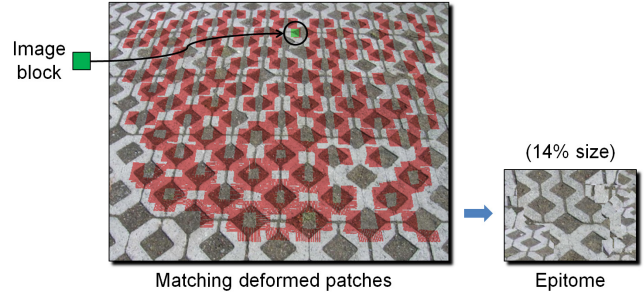
Figure 4: Image blocks match many affinely deformed instances.
