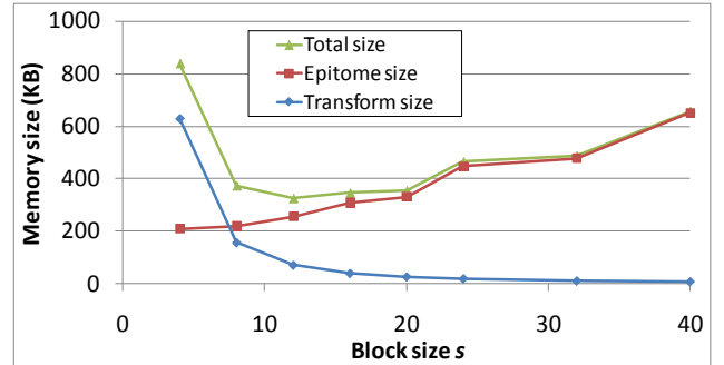
Figure 21: Memory size as function of the image block size s for the example in Figure 1, with fixed error tolerance \epsilon=0.002 .
