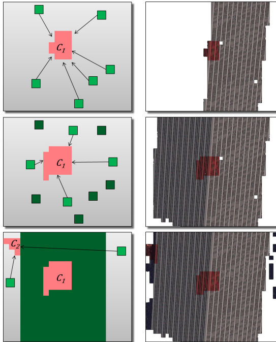
Figure 10: Illustrated example of growing the epitome (in red). The right column reveals the image subset I^E that is accurately reconstructed at each step of the process.
