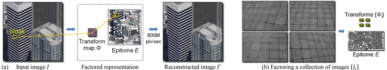
Figure 1: Factoring image content into a block-based transform map and a condensed epitome still allows fast random-access evaluation.
