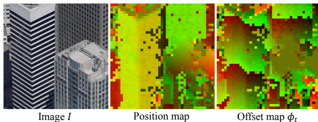
Figure 15: Visualization of the coherence in the transform map. Middle image shows the epitome locations (red= x , green= y ) of the reconstruction, and right image shows translation vectors \phi_t .
