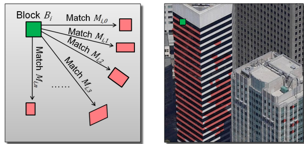
Figure 5: A given image block shown in green accurately matches the transformed patches highlighted in red.
