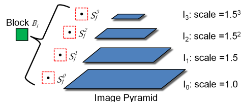
Figure 8: Scaling is handled by searching in pyramid levels.
