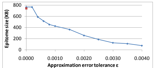
Figure 22: Epitome memory size as function of error tolerance \epsilon for the example in Figure 1, with fixed block size s=12 . The size of the original image (744KB) is indicated by the red square.
