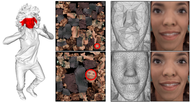
Figure 7: Compared to default results (top row), introducing a surface importance field significantly improves the perceived quality of the reconstructed output frames (bottom row). The importance function, shown in red on the left, is computed automatically using face detection. The sub-images show how adaptive parameterization allocates 4x greater texture atlas area to the face, and how adaptive decimation retains greater geometric detail there.
