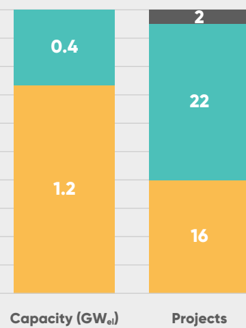
Water electrolysis capacity under construction in Europe by technology
