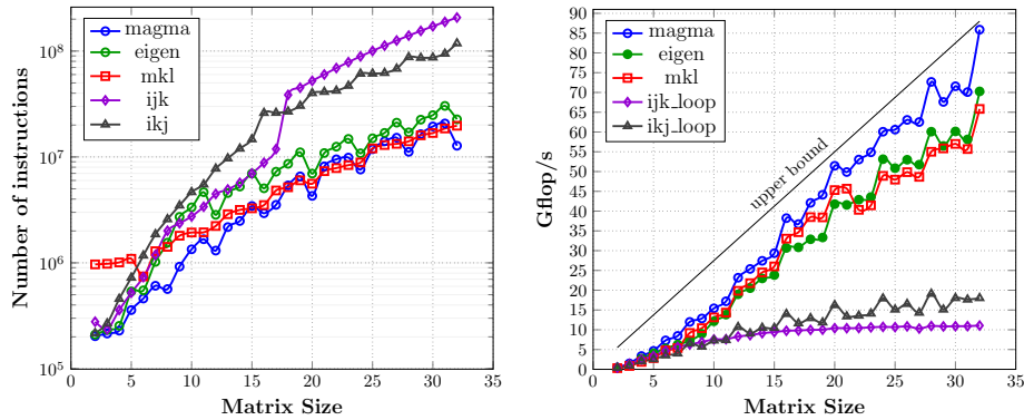
(a) Total CPU instruction count
