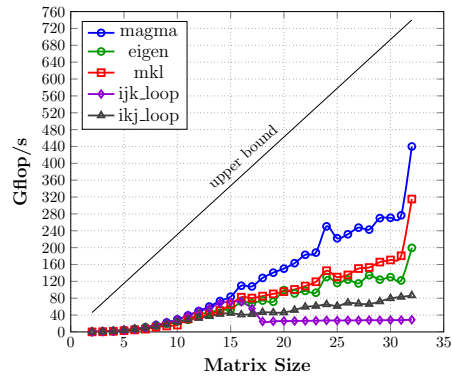
(b) CPU Performance comparison with MCDRAM
