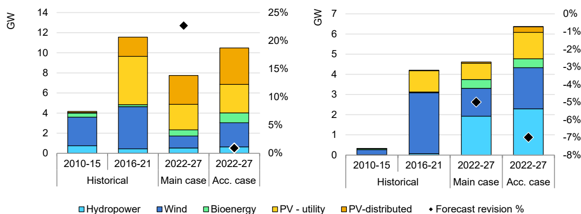
Figure 1.35 Mexico renewable capacity additions, 2010-2027 (left) and Argentina renewable capacity additions, 2010-2027 (right)
