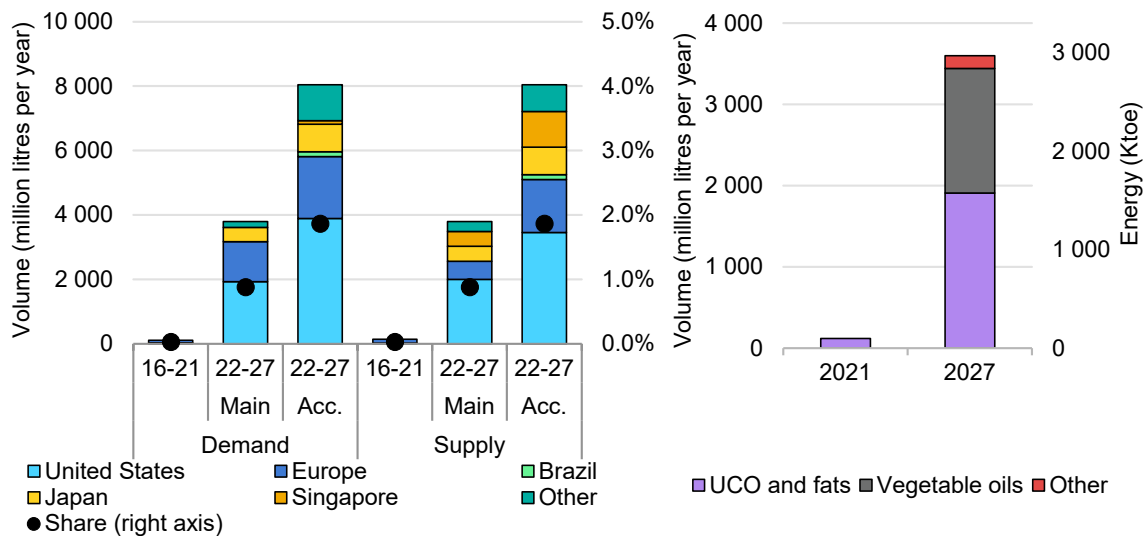
Figure 2.5 Global biojet fuel demand and supply growth, 2016-2027
