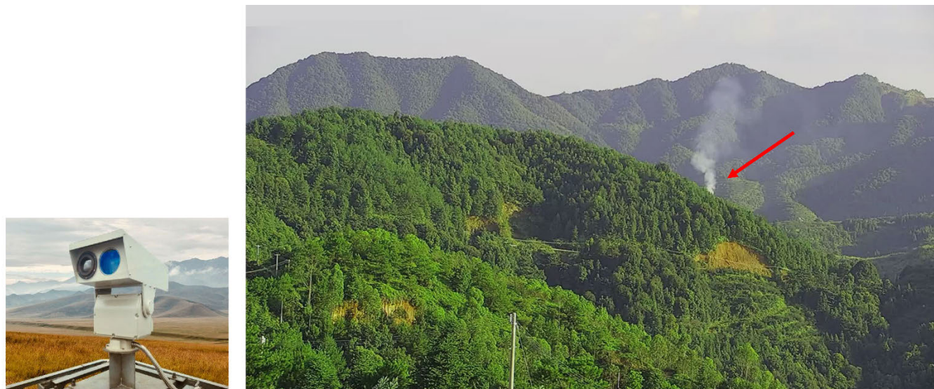
FIGURE 1. A pan-tilt-zoom (PTZ) long range camera for forest fire detection and a snapshot of a typical forest fire smoke at the initial stage captured by a forest watch tower.
