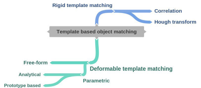
FIGURE 9. An overview of template matching techniques.
