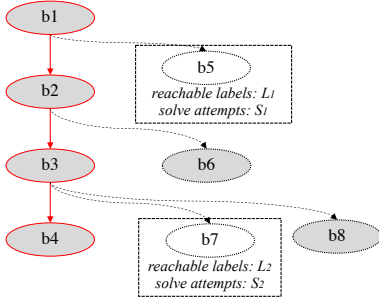
Fig. 3: An example showing how to estimate the bug-detecting potential of a seed. In this example, the seed follows the path b_1 \rightarrow b_2 \rightarrow b_3 \rightarrow b_4 . Basic block b_5 and b_7 are unexplored and they can reach L_1 and L_2 UBSan labels, respectively. They have been attempted by constraint solving for S_1 and S_2 times. The final score for this seed is \frac{e^{-0.05S_1} \times L_1 + e^{-0.05S_2} \times L_2}{2} .
