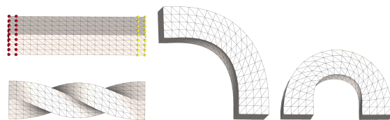
Figure 6: Twist and rotation deformations.
