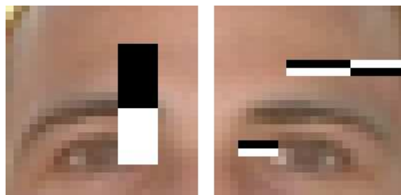
Figure 3. The first three Haar features chosen for AU 1, superimposed on the combined left and right brow regions. Feature 1 (left) is Type 2, Feature 2 (middle) is Type 2, and Feature 3 (right) is Type 4.
