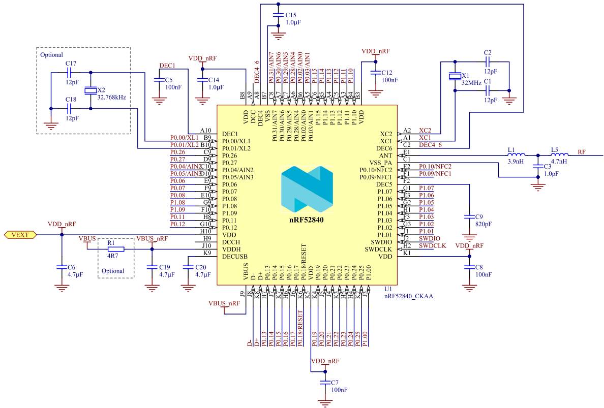
Figure 216: Circuit configuration no. 1 schematic for CKAA WLCSB
