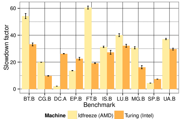
Figure 8: TABARNAC ’s instrumentation overhead.
