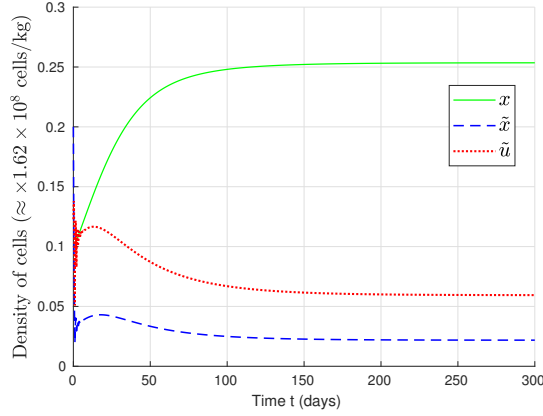
Figure 7: Trajectories of the system of the numerical example 4 (Tables 1-2). In this case, the dormancy steady state \mathfrak{D} exists, such that \tilde{x}_e = 0.0217 , \tilde{u}_e = 0.0593 . The sufficient local stability conditions given in Theorem 2-(B) are satisfied, as shown in (66), and the trajectories of the system converge exponentially to \mathfrak{D} .
