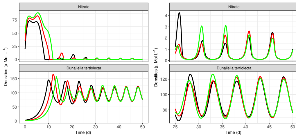
(c) Dynamics with \tau = 1.4 d .
