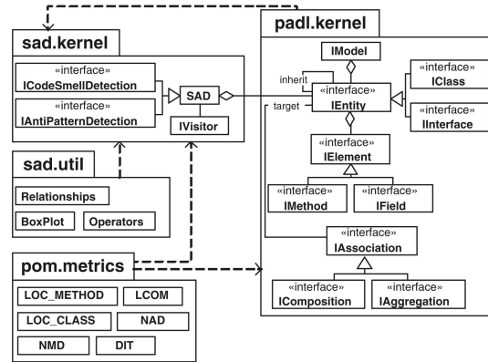
Fig. 8. Architecture of the SMELFW framework.
