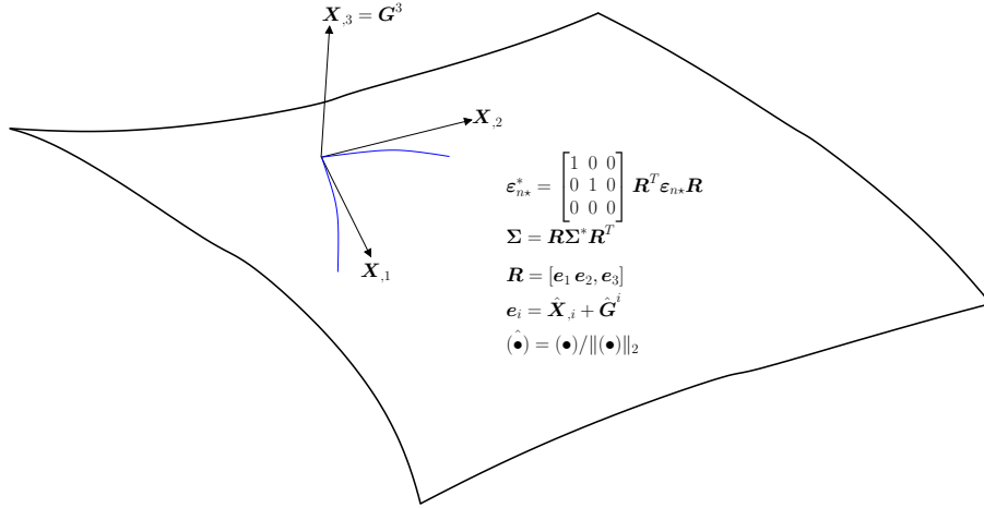
Figure 1. Return mapping: filtering of the normal strain and stress.
