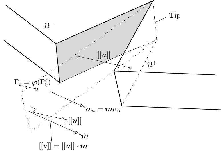
Figure 4. Cohesive forces arising from the crack surface separation.
