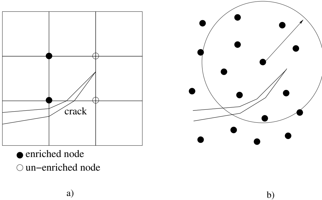
Figure 3. Crack with enriched nodes in XFEM and meshfree methods
