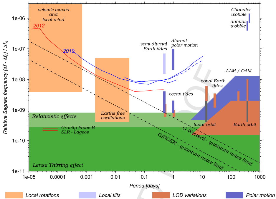
Fig. 2. (Color online.) The picture compares the Allan deviation of G in Wettzell (years 2012 and 2010, courtesy of K.U. Schreiber) with the most relevant geodetic signals. The green parts show the region of interest for the geodetic precession and the Lense–Thirring effect; on the left of the picture it is possible to see the present level of test obtained by Gravity Probe B and Lageos. The two dotted lines show the shot noise of the G (16-m perimeter), and of a ring with perimeter 24 m.
