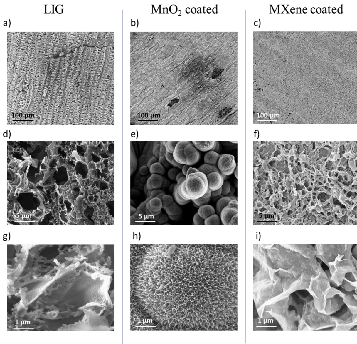
Fig. 2. Micrographs acquired by different magnification at FESEM. LIG images are on the left column. In the middle column \text{MnO}_2 decorated LIG is shown, while in the last column MXene decoration is appreciated. The comparison is proposed at 100 \mu\text{m} scale (a,b,c), 5 \mu\text{m} scale (d,e,f) and 1 \mu\text{m} scale (g-i).
