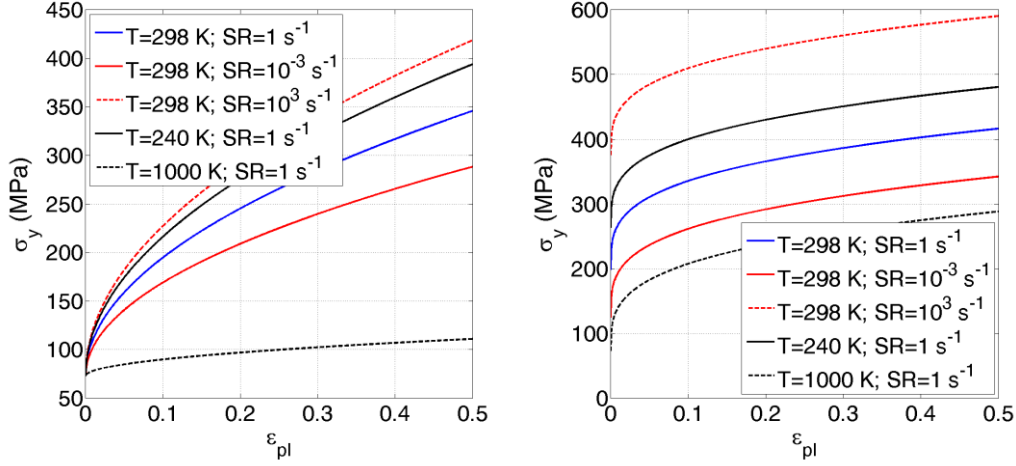
Fig. 4.2: Z-A model for copper (left) and Armco iron (right): effect of strain-rate and temperature variations.
