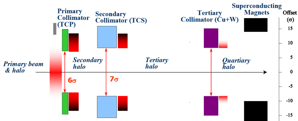
Fig. 7.1: Qualitative scheme of the LHC collimation system.
