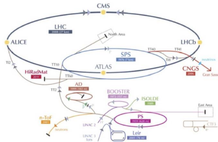
Fig. 8.1: Scheme of the CERN accelerator complex: identification of the HiRadMat site.
