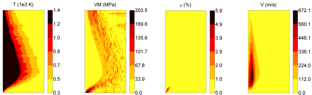
Fig. 6.7 Temperature, Von Mises stress, plastic strain and particle velocity distributions on the copper cylindrical component at the end of the deposition phase: radius 0-10 mm ( \rightarrow ), length 0-1 m ( \uparrow ), the radial dimension is amplified.
