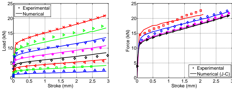
Fig. 4.12: Comparison between experimental data and numerical results for the tests at different temperatures: \times 20^\circ \text{ C} , \triangleright 100^\circ \text{ C} , \nabla 200^\circ \text{ C} , * 300^\circ \text{ C} , \diamond 400^\circ \text{ C} , \triangleleft 500^\circ \text{ C} , \square 600^\circ \text{ C} and \triangle 700^\circ \text{ C} . Comparison between experimental data and numerical results for the tests at different strain-rates (case 2): \square 10^3 \text{ s}^{-1} , \diamond 10 \text{ s}^{-1} , * 10^{-1} \text{ s}^{-1} , \triangleright 10^{-3} \text{ s}^{-1} (right).
