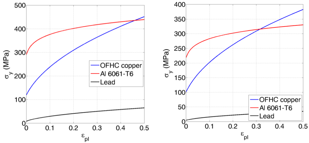
Fig. 4.3: S-G model for FCC materials, such as Al 6061-T6, OFHC (1/2 hard) copper and lead for two different temperatures: 300 K (left) and 700 K (right); \varepsilon_{pl,i} = 0 , P = 0 GPa.
