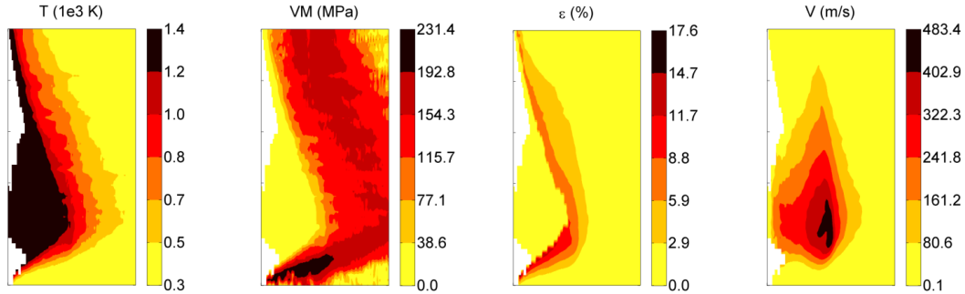
Fig. 6.8: Temperature, Von Mises stress, plastic strain and particle velocity distributions on the copper cylindrical component after 1\mu\text{s} from the impact: radius 0\div 10\text{ mm} ( \rightarrow ), length 0\div 1\text{ m} ( \uparrow ), the radial dimension is amplified.
