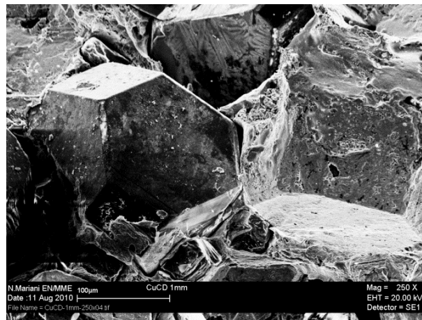
Fig. 8.6: SEM view of CuCD: 175 \mu m diamonds surrounded by the Cu phase. The white spots on diamond surfaces are boron carbides.
