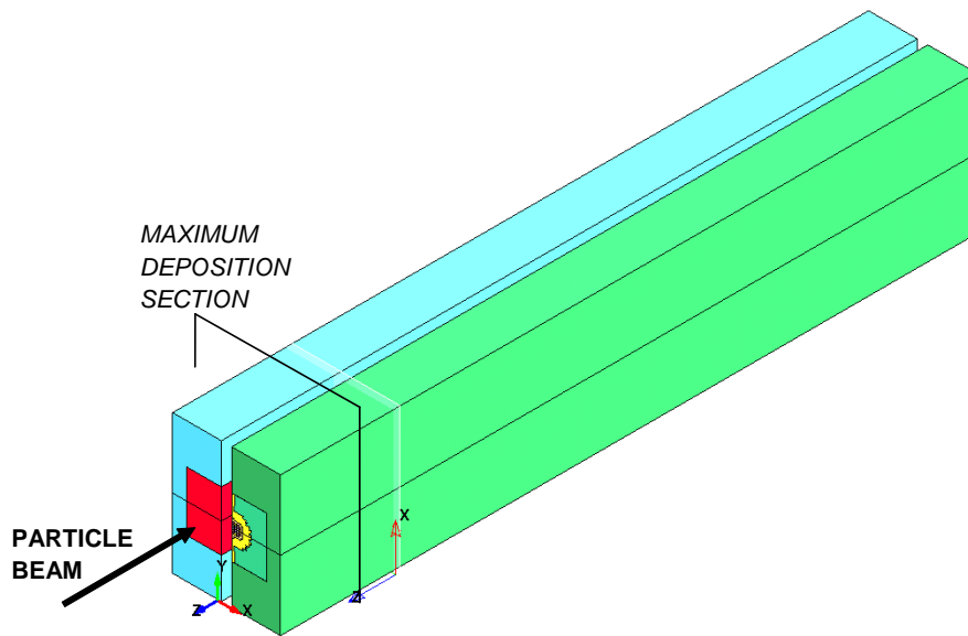
Fig. 7.2: 3D view of the simplified TCT.
