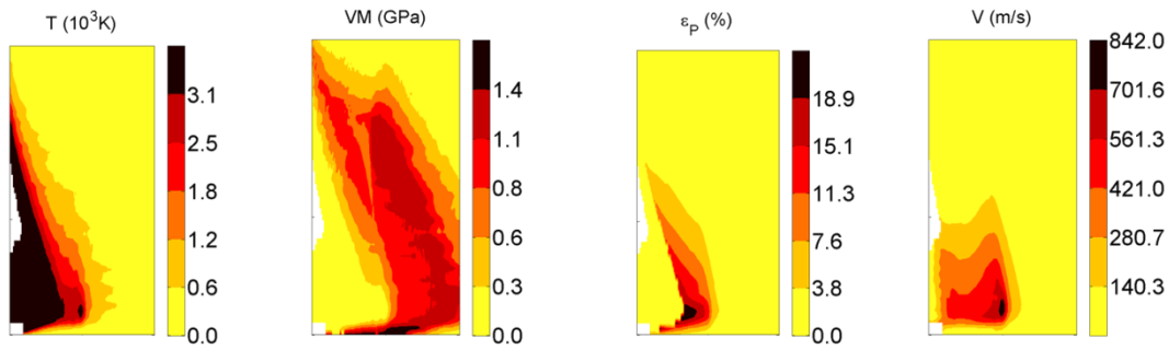
Fig. 6.18: Temperature, Von Mises stress, plastic strain and particle velocity distributions on the tungsten cylindrical component after 1 \mu s from the impact (J-C model): radius 0÷10 mm ( \rightarrow ), length 0÷1 m ( \uparrow ), the radial dimension is amplified.
