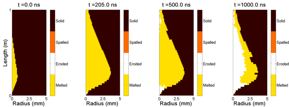
Fig. 6.9: Time evolution of the four type of damage evaluated: fusion, erosion, spallation and cumulative damage on the copper cylindrical component at four different time steps: radius 0\div 5\text{ mm} ( \rightarrow ), length 0\div 1\text{ m} ( \uparrow ), the radial dimension is amplified.
