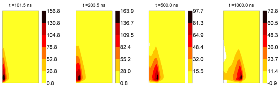
Fig. 6.13 Pressure distribution (GPa) on the tungsten cylindrical component at four different time steps: radius 0÷10 mm ( \rightarrow ), length 0÷1 m ( \uparrow ), the radial dimension is amplified.
