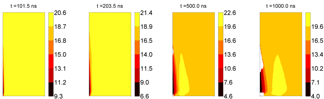
Fig. 6.14 Density distribution ( \text{kg/dm}^3 ) on the tungsten cylindrical component at four different time steps: radius 0÷10 mm ( \rightarrow ), length 0÷1 m ( \uparrow ), the radial dimension is amplified.
