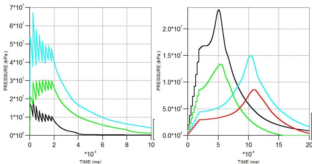
Fig. 6.22: Pressure vs. time history obtained with AUTODYN: (left) for three elements situated along the symmetry axis ( P1 : r=0 mm and L=5 cm; P2 : r=0 mm and L=16 cm; P3 : r=0 mm and L=50 cm) and (right) for four elements situated respectively at P4 : r=2.5 mm and L=20 cm; P5 : r=5 mm and L=20 cm; P6 : r=2.5 mm and L=50 cm; P7 : r=5 mm and L=50 cm.
