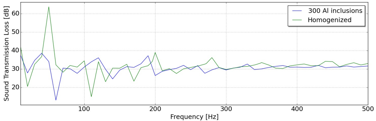
Fig. 4 STL of a simply supported plate, Melamine Foam and 300 Aluminum inclusions (19.2% volume fraction): comparison with equivalent homogenized material
