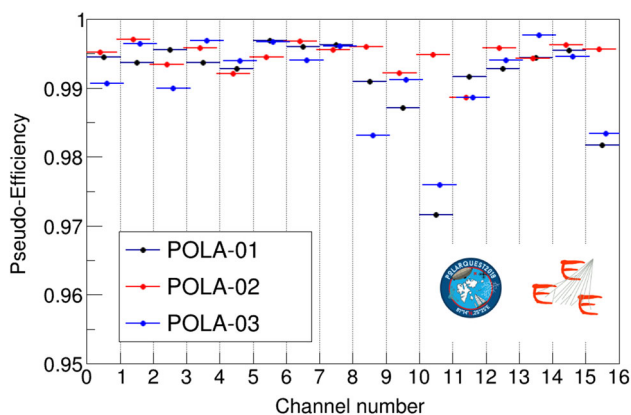
Fig. 12 Channel by channel PE averaged in the full period, for POLA-01, POLA-02 and POLA-03. Here, the binomial errors are used, so small to be visible
