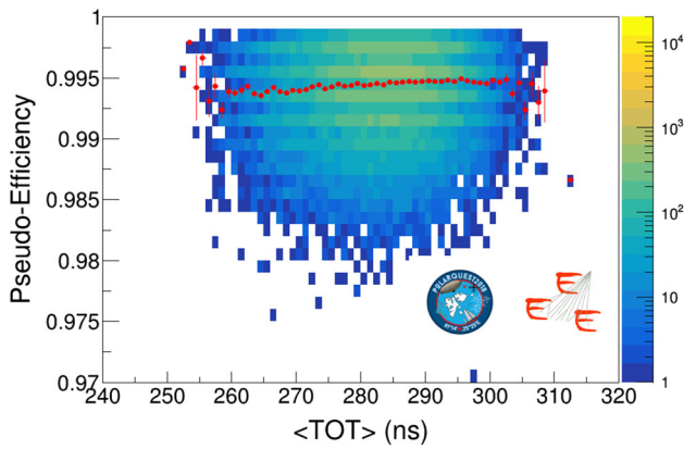
Fig. 14 PE vs. \langle \text{TOT} \rangle for channel-0 of POLA-01. The red points represent the average PE values
