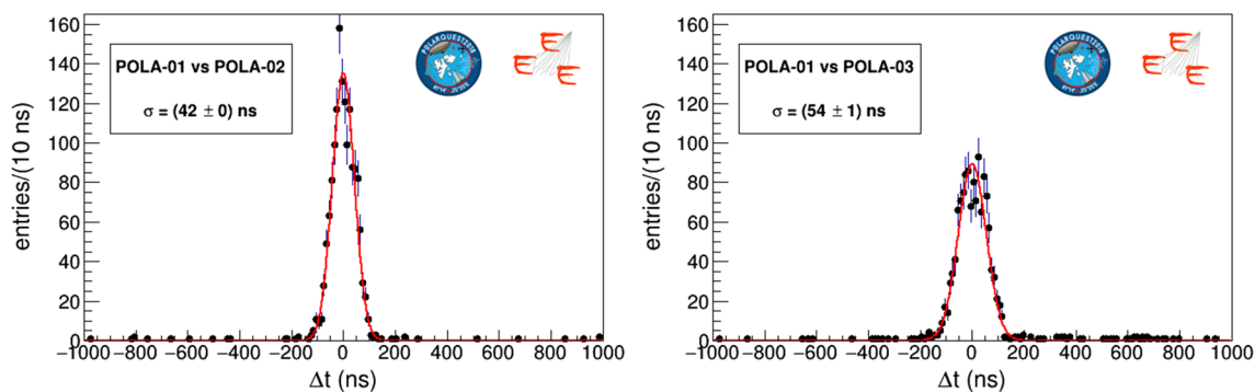
Fig. 9 Time coincidence peaks of POLA-01/POLA-02 (left) and POLA-01/POLA-03 (right). Data were taken on June 17, 2018 and correspond to approximately 2.5 h
