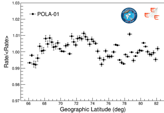
Fig. 25 Rate of cosmic particles, corrected for all the effects mentioned in the previous Section, measured by POLA-01 during its trip in the Arctic Sea
