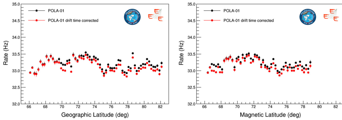
Fig. 28 Rate measured by POLA-01 as a function geographic (left) and magnetic (right) latitude, before (black points) and after long term drift correction (red points)
