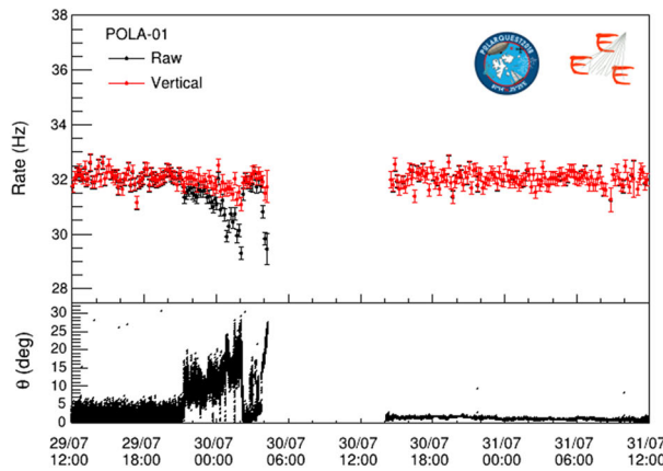
Fig. 20 Left: Raw rate measured by POLA-01 (black points in the upper plot) from July 29 to July 31, 2018, when the boat was inclined for a period of about 9 h. Also the rate corrected for the inclination effect (red points) and the inclination angle (black points in the lower plot) are shown. In this case, a 10 min binning has been used for the rate, while
