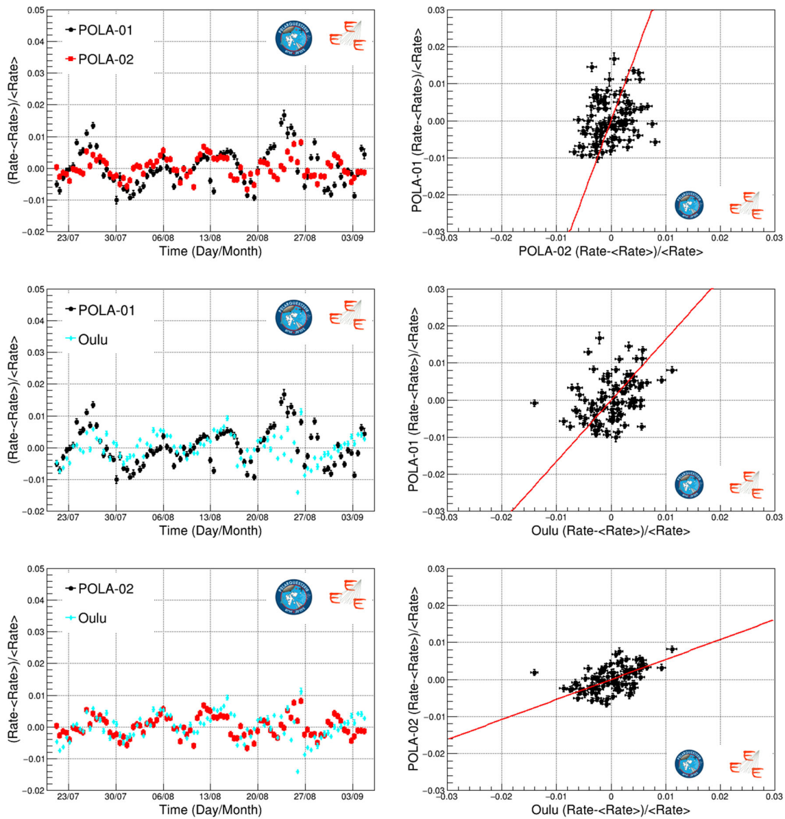
Fig. 30 Percentage rate variations as a function of the time (left column) and rate variation correlation plot (right column). Top row: POLA-01 and POLA-02; middle row: POLA-01 and Oulu; bottom row: POLA-02 and Oulu. The red line shows the fit with a linear function. The
