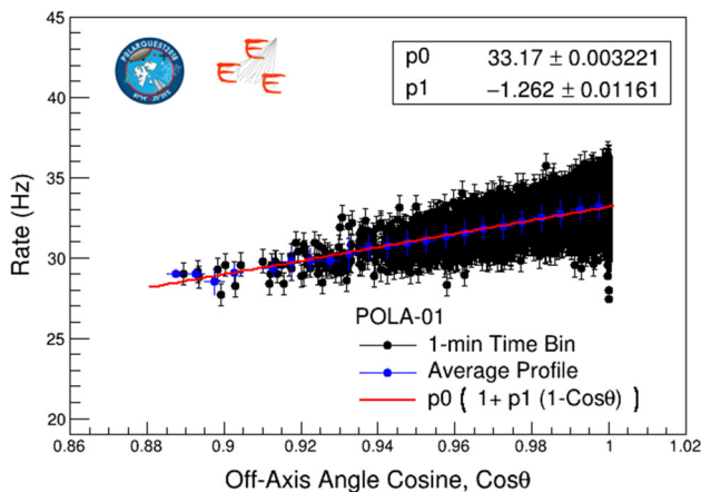
Fig. 19 POLA-01 rate as a function of the cosine of the angle between the vertical and the axis perpendicular to the top surface of the detector
