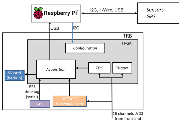
Fig. 4 Read-out DAQ and Control block diagram
