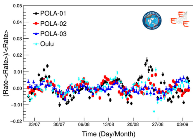
Fig. 29 Percentage rate fluctuations with respect to the average rate measured by the three POLA detectors and by the Oulu neutron monitor, the latter being located at the Sodankylä Geophysical Observatory of the University of Oulu, in Finland, as a function of time
