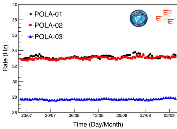
Fig. 23 Rates of cosmic particles measured by the three POLA detectors, corrected for the orientation (POLA-01) and pressure (POLA-01, POLA-02 and POLA-03) effects, as a function time since July 22, 2018
