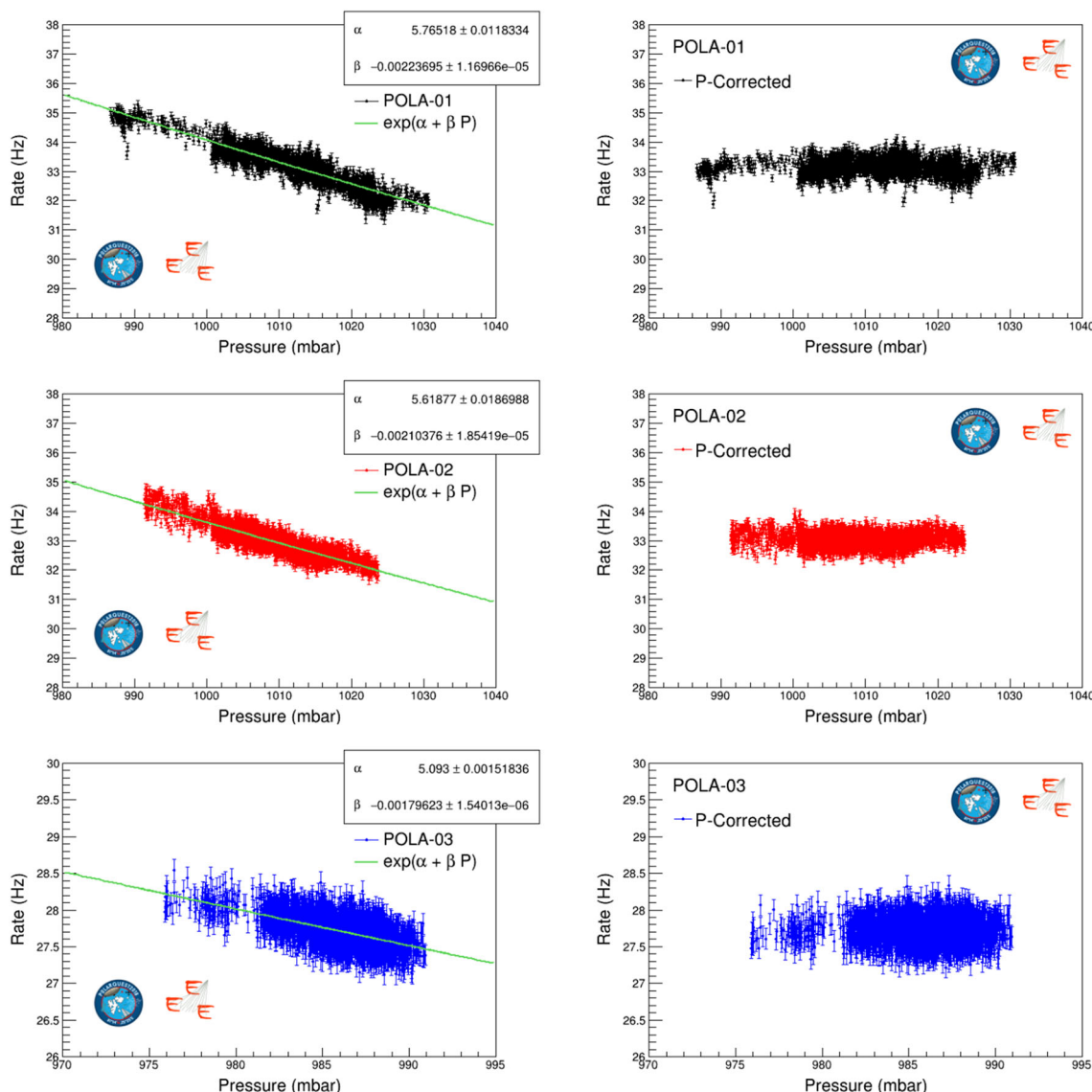
Fig. 22 POLA-01 (top), POLA-02 (middle) and POLA-03 (bottom) rates as a function of the pressure. Left column: rates corrected for the angle with respect to the vertical direction for POLA-01 and raw rate for POLA-02 and POLA-03 (the green line shows the best fit result); right
