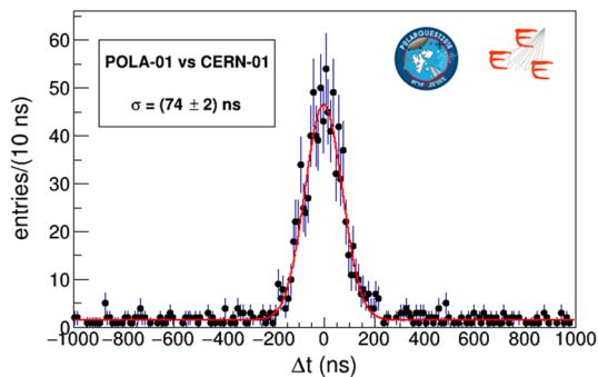
Fig. 8 Time coincidences between POLA-01 and CERN-01; data were taken on the June 17, 2018
