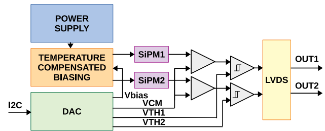
Fig. 2 Simplified block diagram of the FE card, showing its main components
