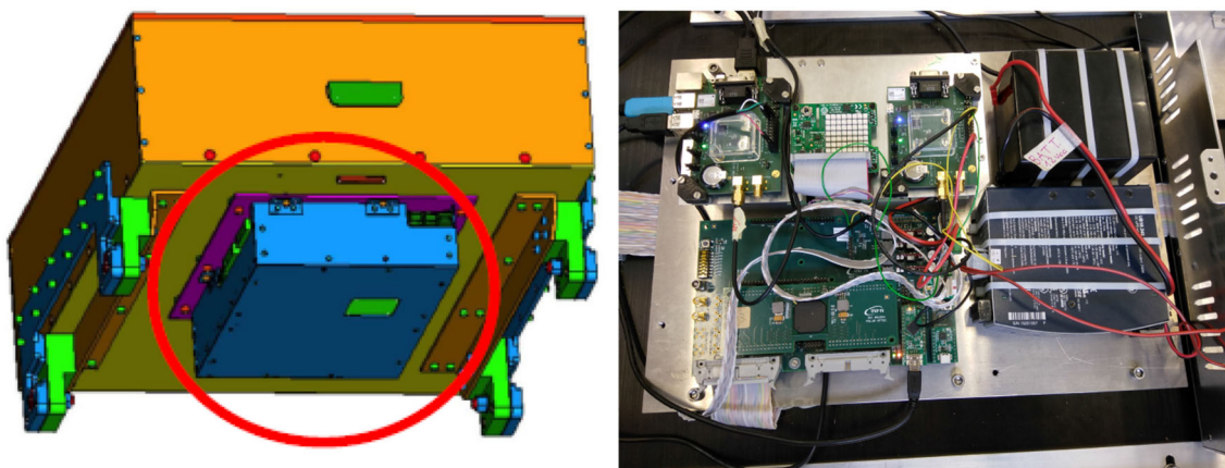
Fig. 3 Left panel: artist view of the detector box, with the electronics box at the bottom (highlighted with a red circle). Right panel: electronics box with the TRB, the power supply, the RPi3, the Sense Hat and the EVK-M8xZOE GLONASS board
