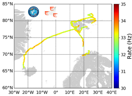
Fig. 25 Rate of cosmic particles, corrected for all the effects mentioned in the previous Section, measured by POLA-01 during its trip in the Arctic Sea
