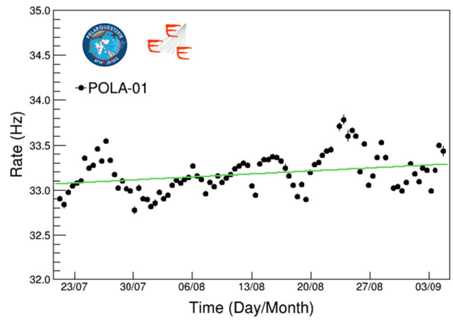
Fig. 25 Rate of cosmic particles, corrected for all the effects mentioned in the previous Section, measured by POLA-01 during its trip in the Arctic Sea
