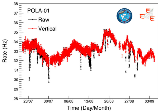
Fig. 21 POLA-01 rate as a function of time from July 22 to September 4, 2018. Black points: raw rate; red points: rate corrected for the inclination effect discussed in the text
