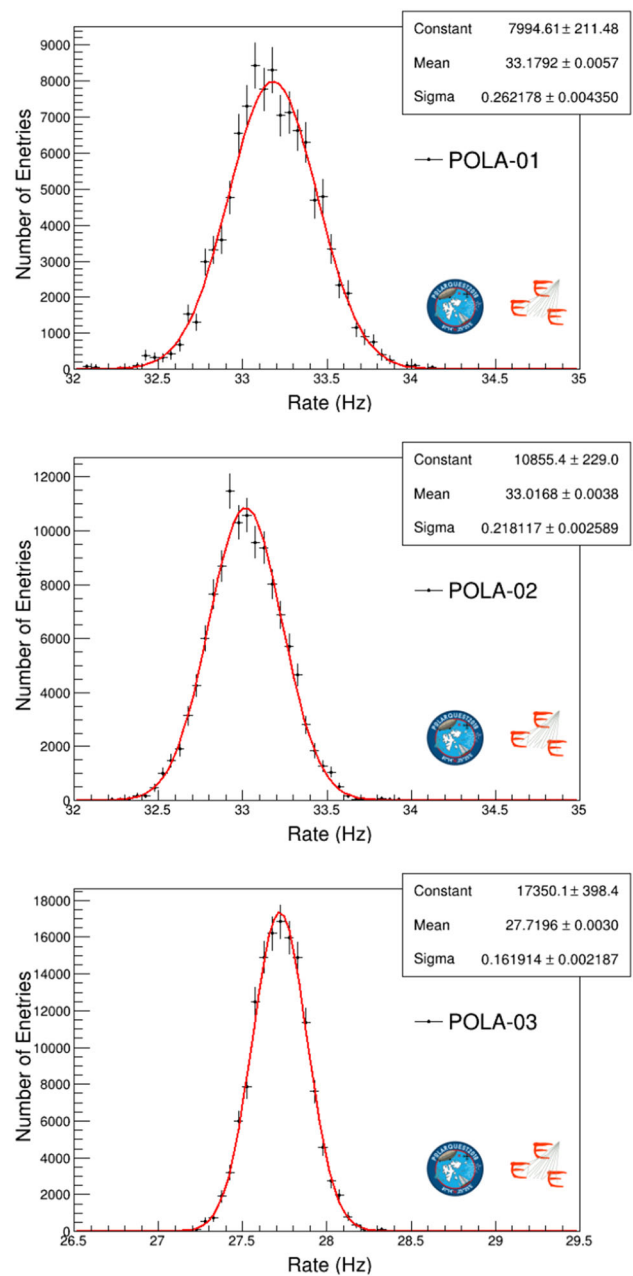
Fig. 24 Distributions of the rate observed by the three POLA detectors during data taking, with Gaussian fits superimposed
