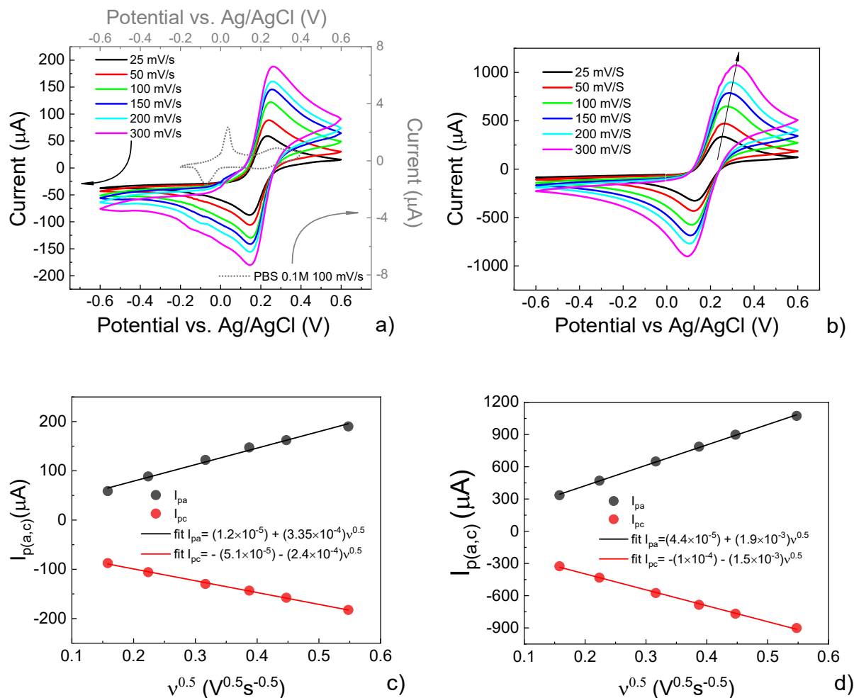
Figure 1: Cyclic voltammetry of Potassium Ferricyanide (K 3 [Fe(CN) 6 ]), 25 mM, in PBS (pH 7.4), 100 mM (scan rates 25, 50, 100, 150, 200 and 300 mV/s) carried out using (a) a SPE equipped with Au working and counter electrodes and Ag/AgCl reference electrode; (b) the same measurement as in (a) using a homologue SPE where the working electrode is covered by a PEGDA:PEDOT layer; (c) anodic and cathodic peak positions extracted from (a) as a function of the square root of the scan rates (related fitting curves, solid lines); (d) anodic and cathodic peak positions extracted from (b) as a function of the square root of the scan rates (related fitting curves, solid lines).
