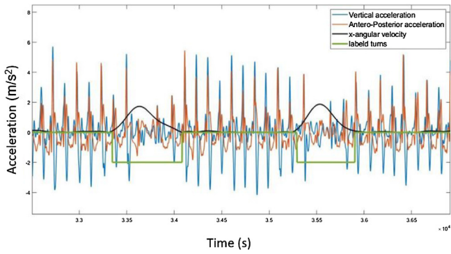
Fig. 2. Acceleration and angular velocity signals related to walking and turning activities. For better visualization, the x -component of angular velocity was low-pass filtered ( f_c = 0.5 Hz), removing high frequency noise. (For interpretation of the references to color in this figure legend, the reader is referred to the web version of this article.)
