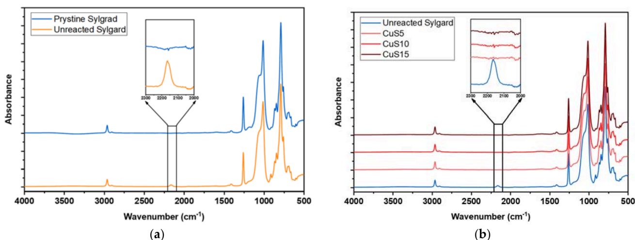
Figure 1. ATR-FTIR spectra; (a) spectra of Sylgard pristine formulation (Entry 1; Table 1) before (orange curve) and after (blue curve) thermal curing at 150 °C. zoom of the Si-H peak at 2160 cm -1 in the insert of the graph; (b) spectra filled Sylgard formulation containing spheroidal Cu (Entry 2, 3, 4; Table 1), before (blue curve) and after (red curves) thermal curing at 150 °C. Zoom of the Si-H peak at 2160 cm -1 in the insert of the graph.
