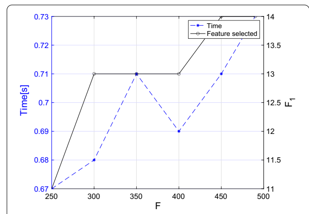
Fig. 7 Execution time of the algorithm with different numbers of input features. The final number of features selected is also reported
