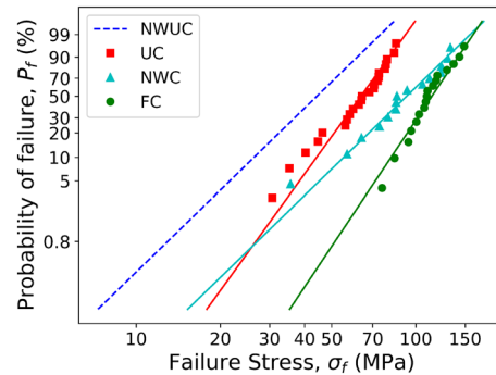
Fig. 11 Weibull distribution functions for the bending strength of un-coated (UC), freshly coated (FC), and naturally weathered coated (NWC) glass samples
