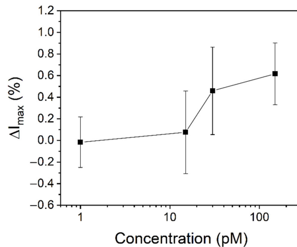
Figure 5. Differential channel current variation with the BSA concentration in PBS 1×. The error bars are calculated on at least three different devices.
