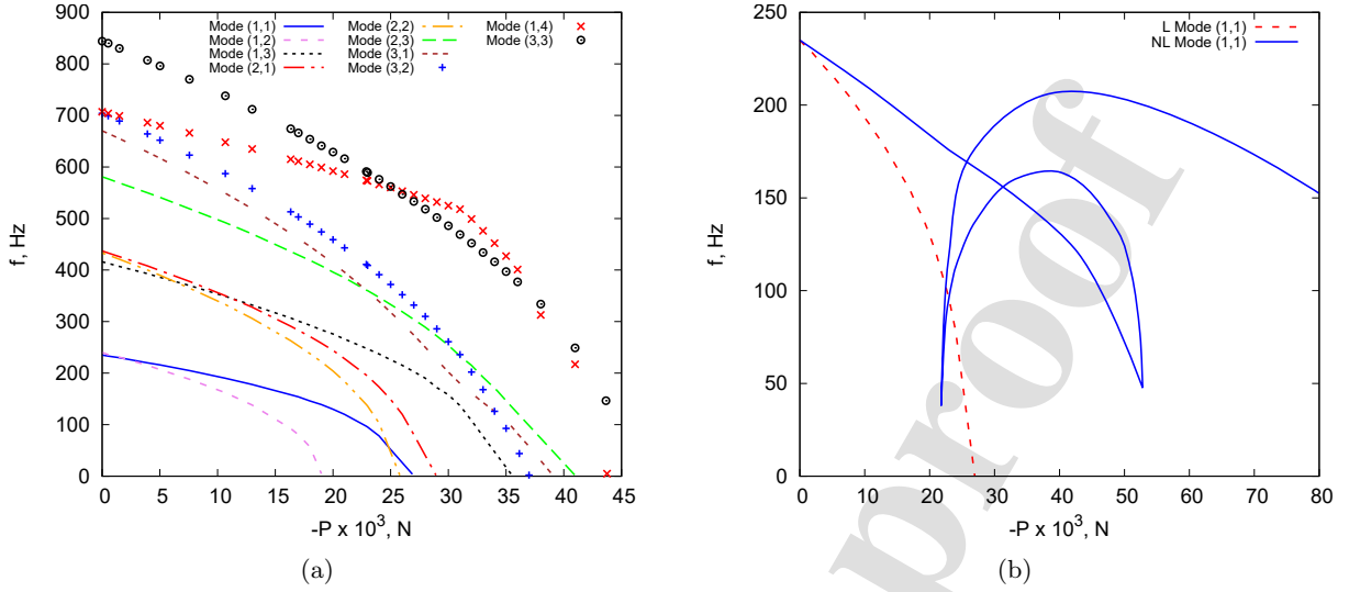
Figure 13: Natural frequency variation versus compressive loading via (a) trivial linearized solution and (b) full nonlinear solution (NL) vs trivial linearized solution (L) for mode (1,1). Curved panel with R/a=5 .
