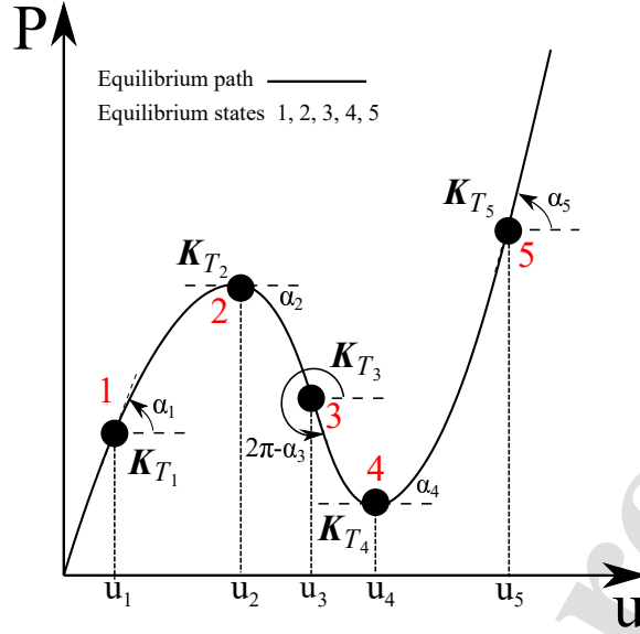
Figure 3: K_T for representative states of equilibrium of a generic nonlinear equilibrium curve.
