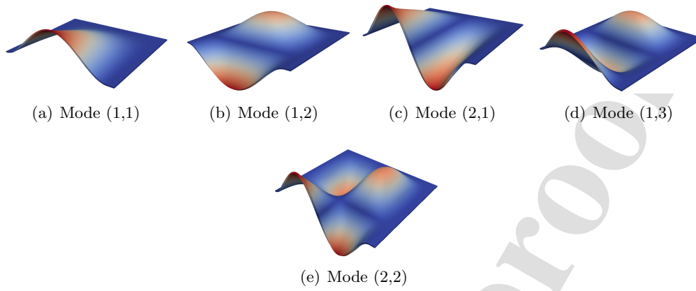
Figure 8: Characteristics first five free vibration mode shapes for the aluminium plate 2.
