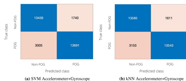
Figure 5. Performance of subject-independent algorithm with multi-modal classification, using left lateral tibial accelerometer and gyroscope. (a) Confusion Matrix obtained with SVM. (b) Confusion Matrix obtained with kNN.
