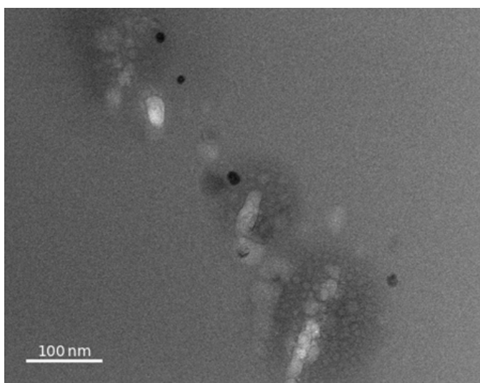
Figure 6: TEM image of bubbles/cavities in the irradiated portion of the CA sample irradiated at 710°C.
