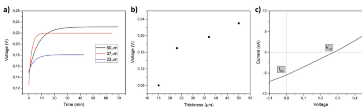
Figure 5. Electrical and electrochemical results varying the membrane thickness. a) OCP variation in time (original data in Figure S5, Supporting Information). b) OCP values obtained at different thicknesses. c) IV curve for the most performant membrane (50 μm).
